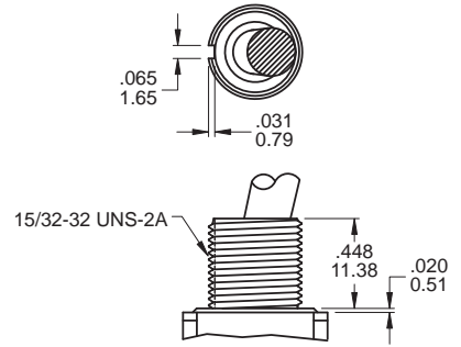
Use with T7, T8 actuators only B13 Bear strength from top of actuator up to 10kg aside up to 15kg
