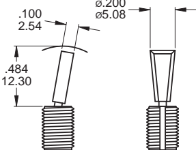
T6 FLATTED WITH ANTIROTATION
